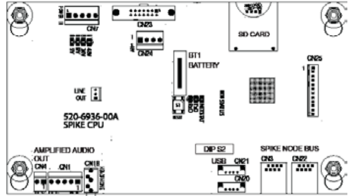
Figure 3.3.6. SPIKE CPU Node connector detail.
