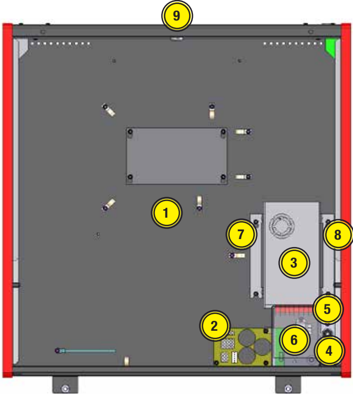
Figure 5.10.3. Backbox internal assemblies and components
