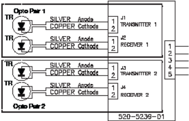
Figure 4.13.4. Opto amplifier 500-5239-01 scehmatic.
