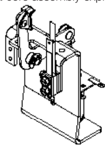
Figure 5.42.5. Sling shot core assembly explosion.
